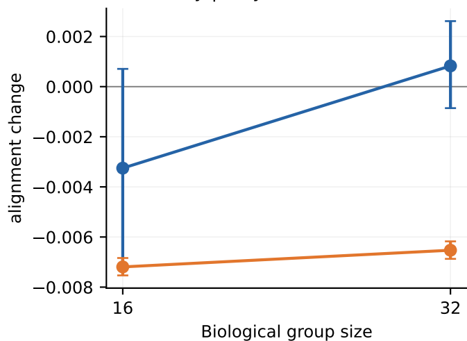
Prey | Prey reorientation R
