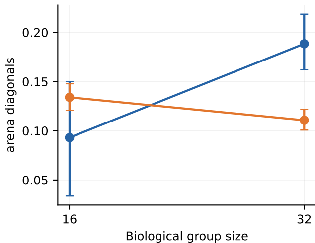
Predator | Predator distance
