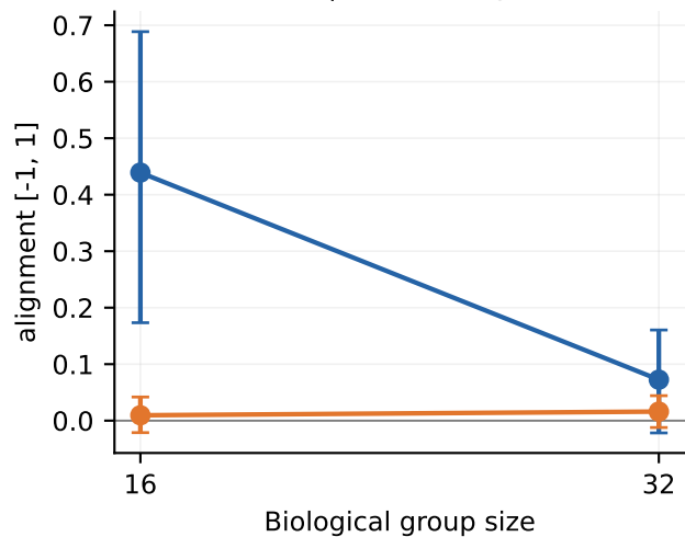
Predator | Pursuit alignment
