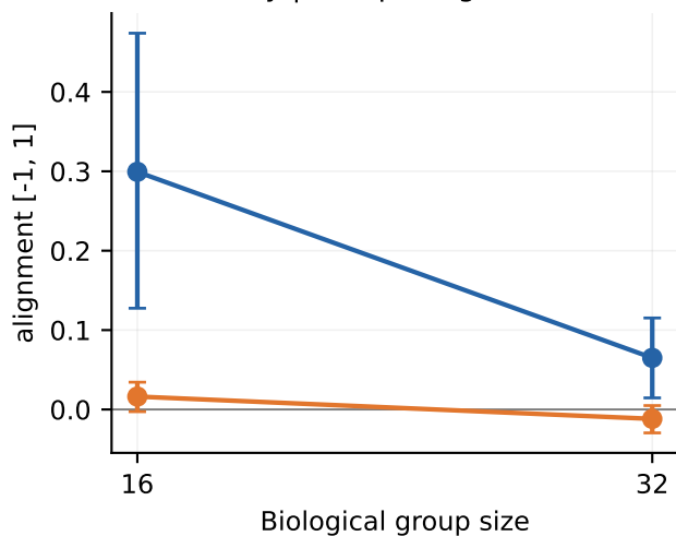
Prey | Escape alignment
